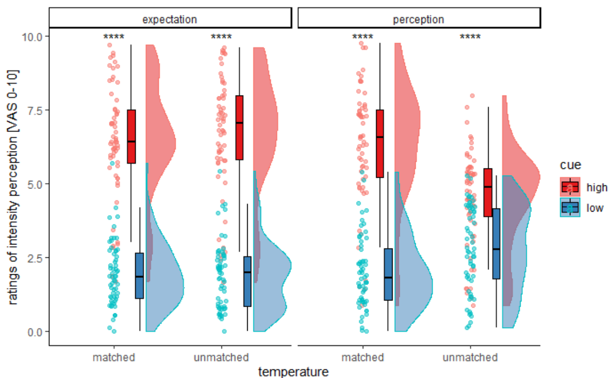
Figure 43. Averaged ratings of expected and perceived intensity of stimulation, given before and after each stimulus. The ratings were converted to a scale from 0-10 for readability. Matched conditions: low cue + low intensity stimulation, high cue + high intensity stimulation: unmatched conditions: low cue + medium intensity stimulation, high cue + medium intensity stimulation. Pairwise comparison; p<0.0001 :****.
